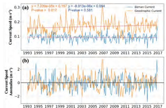
Figure 3. Monthly (a) mean, and (b) anomalies of, geostrophic and Ekman current speeds ( \text{m s}^{-1} ) around the PEIs. Dotted lines show a small positive linear trend ( P < 0.05 ) for geostrophic but not Ekman currents ( P > 0.05 ).
