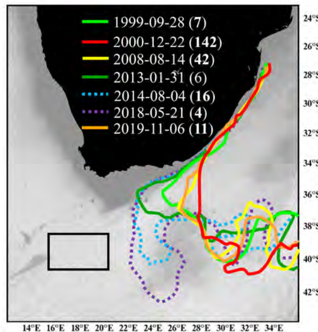
Figure 2. Composite illustration of all early retroflexion events. Solid lines indicate early retroflexions (east of 22.54°E) while the dashed lines indicate events associated with Agulhas Ring shedding. The bold number in parentheses indicates the total length in days of each event. The black box shows the long-term average location of the Agulhas Retroflexion.
