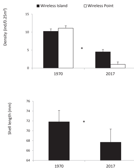
Figure 2. Reductions in mean (+ standard error) densities (top panel) and sizes of the C. granatina between 1970 and 2017 at two sites near Kommetjie where harvesting has increased due to growing coastal developments. Stars indicate statistically significant differences.
