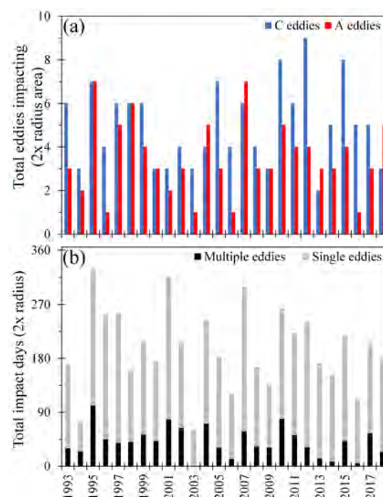
Figure 3. Total number of (a) cyclonic (C) and anticyclonic (A) eddies, and (b) days per year, when their impact area (2 x radius) intersected the 1 000 m isobath of the PEI shelf.
