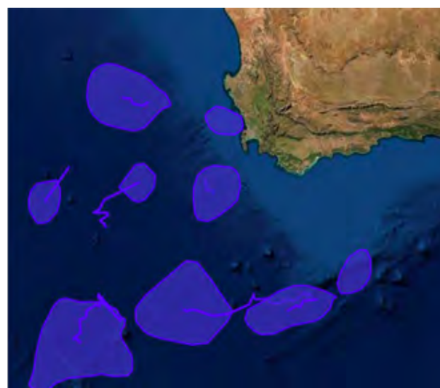
Figure 1. Top: The cyclonic (blue contours) and anticyclonic (red contours) mesoscale eddies detected by the ‘py-eddy-tracker’ on 26 January 2021. Eddy contours are overlaid onto the Absolute Dynamic Topography of the region. Bottom: Selected cyclonic eddies (blue polygons) on 26 January 2021 and their associated historical tracks (blue lines).
