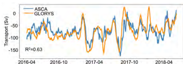
Figure 1. Volume transport time series, spanning April 2016–June 2018, based on the current observations made by the ASCA mooring array (blue), and derived from the GLORYS model (orange). The x-axis labels are year-month.
