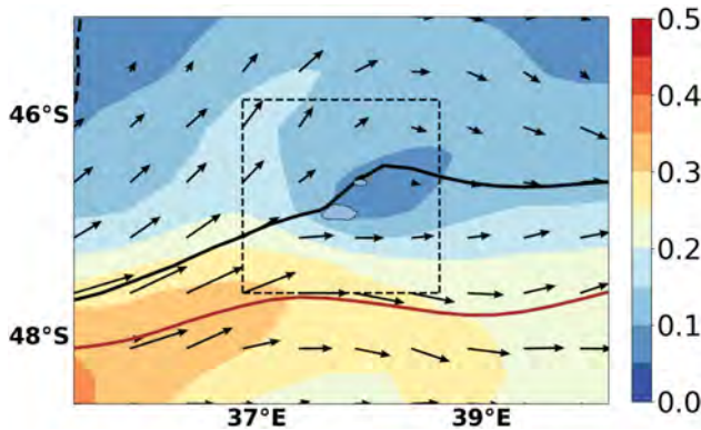
Figure 1. Long-term (1993–2016) mean geostrophic current speed ( \text{m s}^{-1} ) around the PEIs. The dotted black box indicates the 2^\circ \times 2^\circ area ( 45.875\text{--}47.625^\circ\text{S} ; 36.875\text{--}38.625^\circ\text{E} ) around the islands within which satellite data were averaged. The solid black contour indicates the southern branch of the sub-Antarctic Front (S-SAF) and the solid brown contour indicates the northern branch of the Antarctic Polar Front (N-APF).
