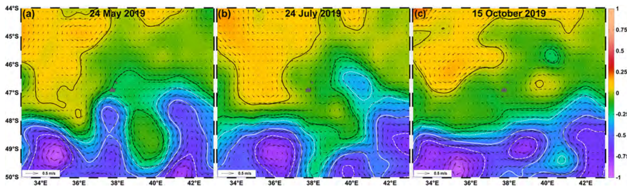
Figure 3. Selected satellite sea surface height (m) maps with geostrophic current vectors. The middle (M-SAF) and southern (S-SAF) branches of the sub-Antarctic Front are indicated by black solid/dashed contours, and the northern (N-APF), middle (M-APF), and southern (S-APF) branches of the Antarctic Polar Front are indicated by white dotted/solid/dashed contours.
