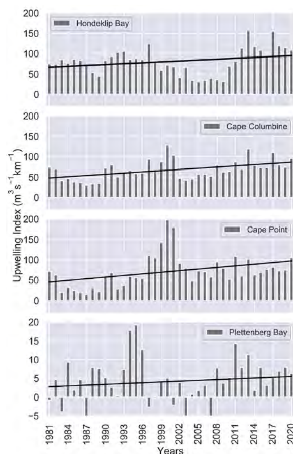
Figure 2. Time series of DJF upwelling index values at four upwelling locations during 1981–2020, with linear trendlines.
