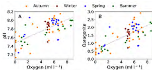
Figure 3. The correlations between (A) pH and dissolved oxygen ( \text{pH} = 7.47 + 0.07 \times \text{Oxygen} ), and (B) aragonite saturation state ( \Omega aragonite) and dissolved oxygen ( \Omega aragonite = 0.57 + 0.19 \times \text{Oxygen} ).
