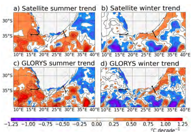
Figure 2. Seasonal linear trend of SST during summer (December–February) and winter (June–August), based on GLORYS model and satellite data. Black lines indicate the ACT/ASCA and SAMBA arrays off the east and west coasts of South Africa, respectively.
