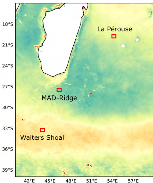
Figure 2. Location of the study sites on a map of seasonal variability in surface Chlorophyll a concentration. Low variability is shown in green and high variability in red colours.
