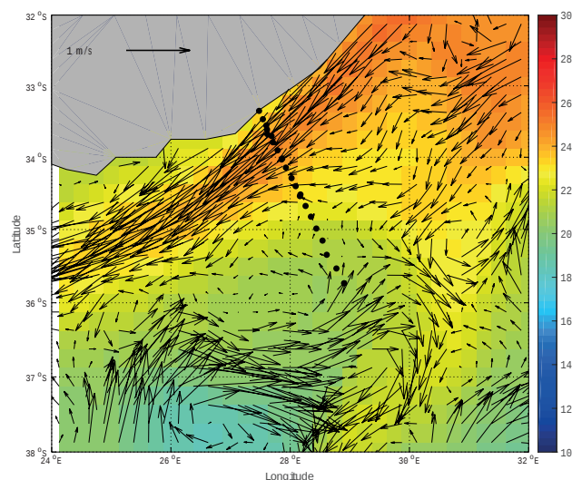
Figure 1. Location of sampling stations along a transect crossing the Agulhas Current, superimposed on a satellite image of Sea Surface Temperature (SST; °C), with current velocity ( \text{m s}^{-1} ) vectors overlaid.
