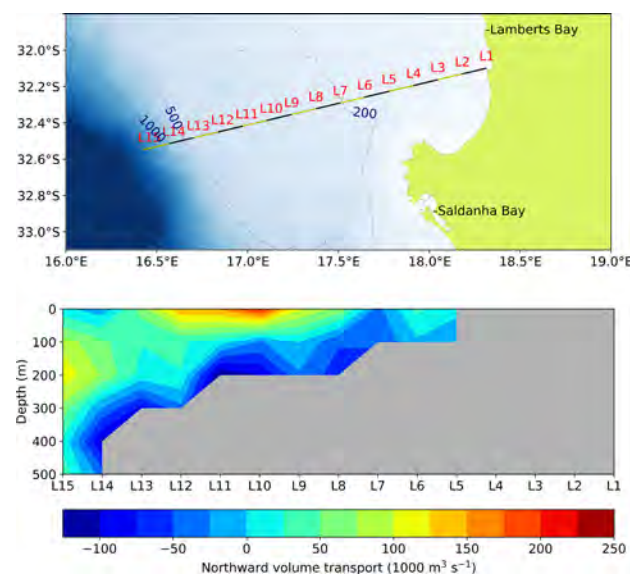
Figure 2. (a) Location of the St Helena Bay Monitoring Line (yellow and black line) as well as the segments, labelled in red, off the west coast of South Africa; (b) northward volume transport for the upper ocean layer along the St Helena Bay Monitoring Line during November 2019.
