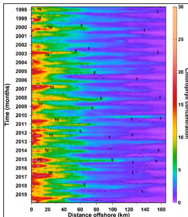
Figure 2: Time series of monthly chlorophyll a ( \text{mg m}^{-3} ) along the St Helena Bay Monitoring Line between 1997 and 2019
