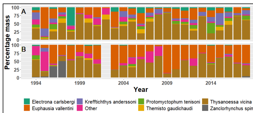
Figure 3: The relative contributions by mass of the dominant prey species in the diet of macaroni (A) and rockhopper penguins (B)
