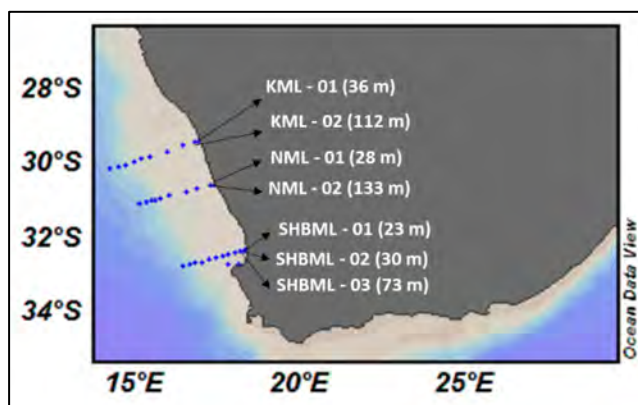
Figure 2: Map showing the Kleinsee (KML), Namaqua (NML) and St Helena Bay (SHBML) monitoring lines of the SB: IEP, and the locations of inshore stations for which pH was determined
