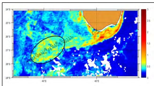
Figure 1: Map of stations sampled on the southern Madagascar shelf and transecting a cyclonic eddy during July 2013, superimposed on a seven-day (13–20 July 2013) composite of Chlorophyll a concentration from MODIS. The black ellipse indicates the approximate boundary of the eddy
