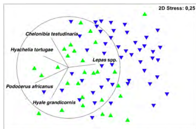
Figure 3: An ordination plot showing differences in turtle epibiont communities between coastal (green) and oceanic foraging turtles, where each point represents a turtle and the proximity between points reflects how similar their epibiont communities were. The black lines indicate in which direction these differences were influenced by the five most diagnostic epibiont species
