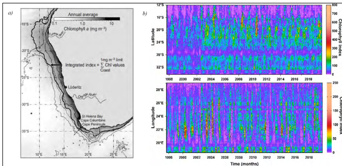
Figure 1: a) Annual average chlorophyll a concentration and location of the 1 mg m -3 contour (thick line), b) Monthly chlorophyll indices (1997–2019) for the west coasts of Namibia and South Africa (top panel) and for South Africa's South Coast (bottom panel)
