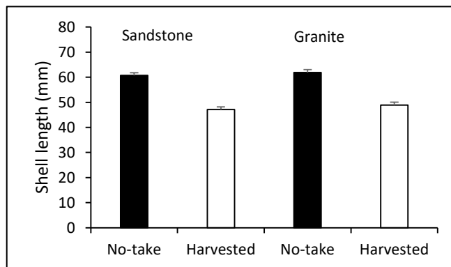
Figure 2: Mean shell lengths (+SE) of C. granatina , in relation to protection level and rock type
