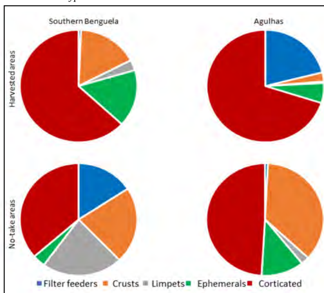
Figure 3: Differences in community composition between harvested vs. no-take areas of the Southern Benguela and Agulhas ecoregions, which make up the western and eastern parts of the MPA, respectively
