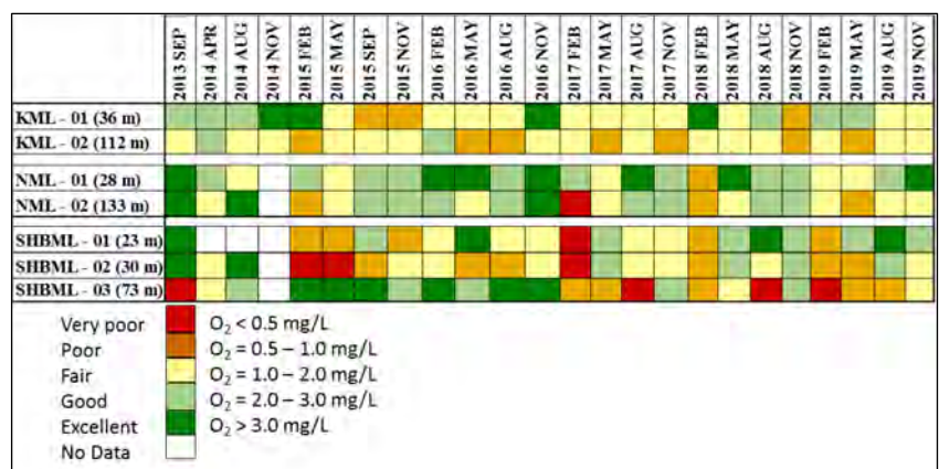
Figure 3: Indicators of oxygen conditions in bottom waters of inshore stations, from 2013–2019
