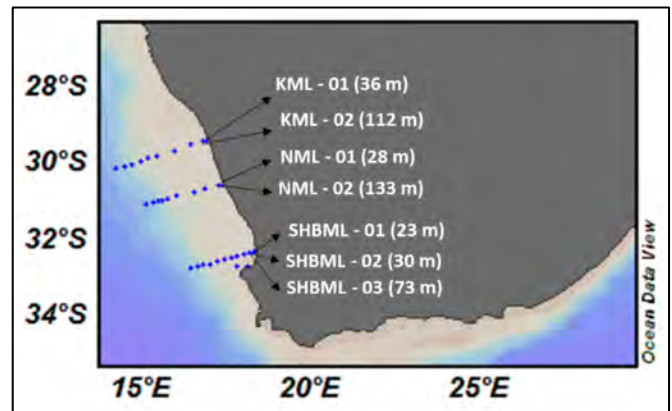
Figure 2: Map showing the Kleinsee (KML), Namaqua (NML) and St Helena Bay (SHBML) monitoring lines of the SB: IEP, and the locations of inshore stations for which oxygen was determined
