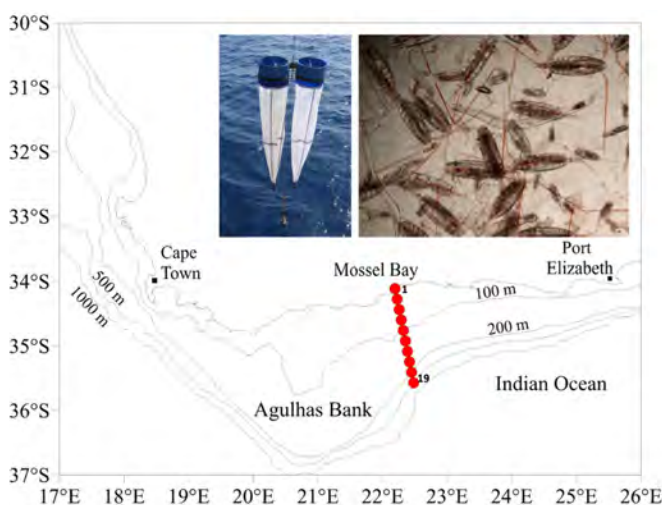
Figure 1: Location of sampling stations 1-19 along the Mossel Bay monitoring line (MBML) on the Agulhas Bank. The inserts show a Bongo net used for sampling, and copepods
