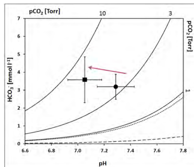
Figure 3: Henderson-Hasselbalch (pH-bicarbonate) diagram for haemolymph of Normocapnic (●) and Hypercapnic (■) seawater. Values are means \pm SD ( n = 12 ). The red arrow indicates a non-compensated respiratory acidosis, i.e. no relevant elevation of bicarbonate ion ( \text{HCO}_3^- ) levels to retain internal pH at pre-incubation/Normocapnic levels
