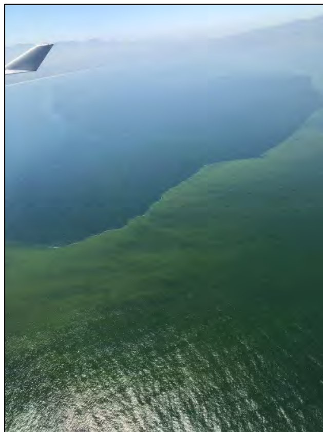
Figure 1: Algal bloom in False Bay on 19 November 2018
