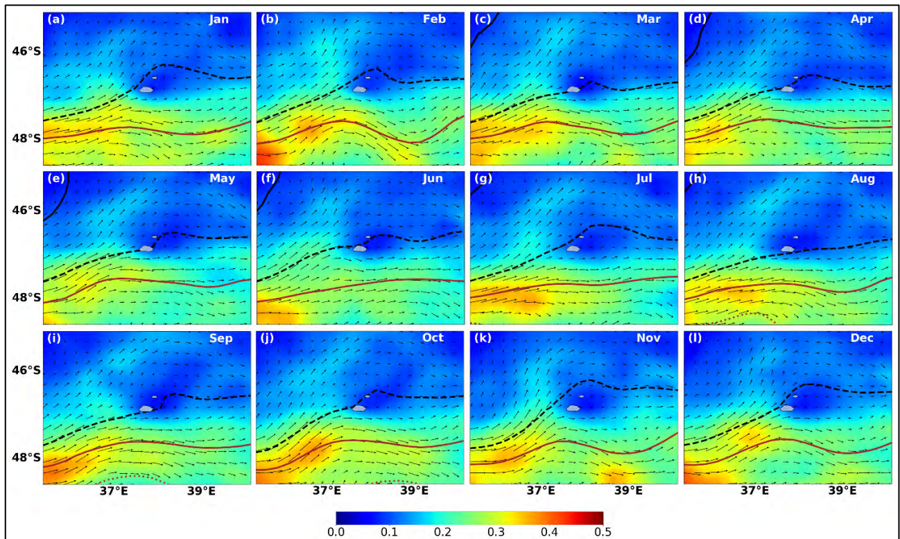
Figure 1: Monthly climatology of geostrophic velocity ( \text{m s}^{-1} ), with vectors indicating the direction of flow, around the PEIs. The solid/dashed black lines show the positions of middle/southern branches of the sub-Antarctic Front (M-SAF/S-SAF), and the solid/dotted brown lines indicate the northern/middle branches of the Antarctic Polar Front (N-APF/M-APF)
