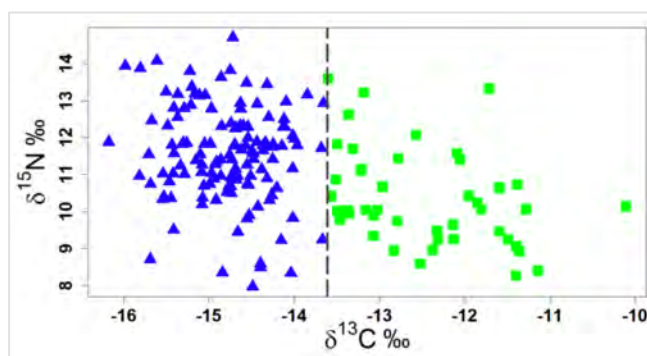
Figure 2: Distribution of carbon ( \delta^{13}\text{C} ) and nitrogen ( \delta^{15}\text{N} ) stable isotope signatures from nesting loggerhead turtles. Two clusters emerged based on carbon isotope ratios, a depleted cluster (blue triangles), and an enriched cluster (green squares), which reflect open-ocean vs coastal feeding, respectively
