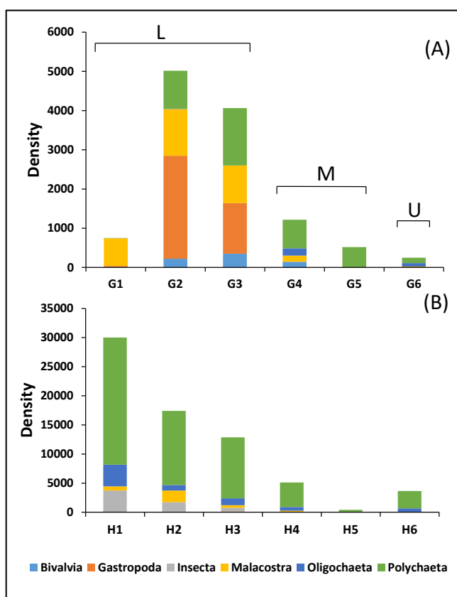
Figure 2: Densities (abundance/m²) of benthic invertebrate classes at the Goukamma (A) and Hartenbos estuaries (B); L = Lower reaches, M = Middle reaches and U = Upper reaches
