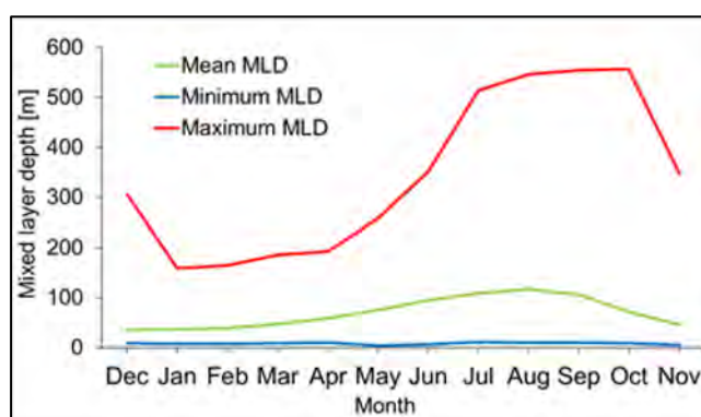
Figure 2: Monthly values of the MLD based on temperature-based criteria obtained from Argo floats
