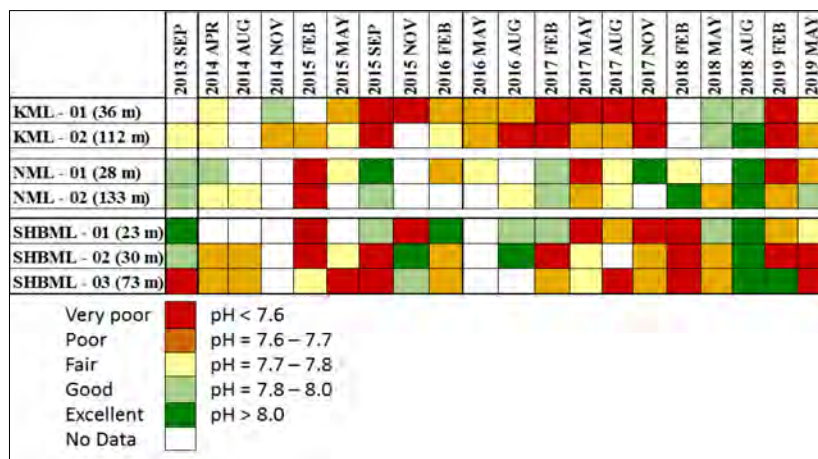
Figure 3: Indicators of ocean pH conditions in bottom waters of inshore stations, from 2013–2019
