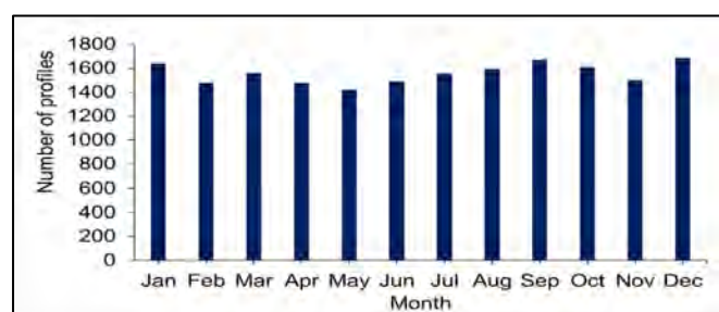
Figure 1: The monthly total of the number of Argo profiles that were used over the study period (2008–2018)
