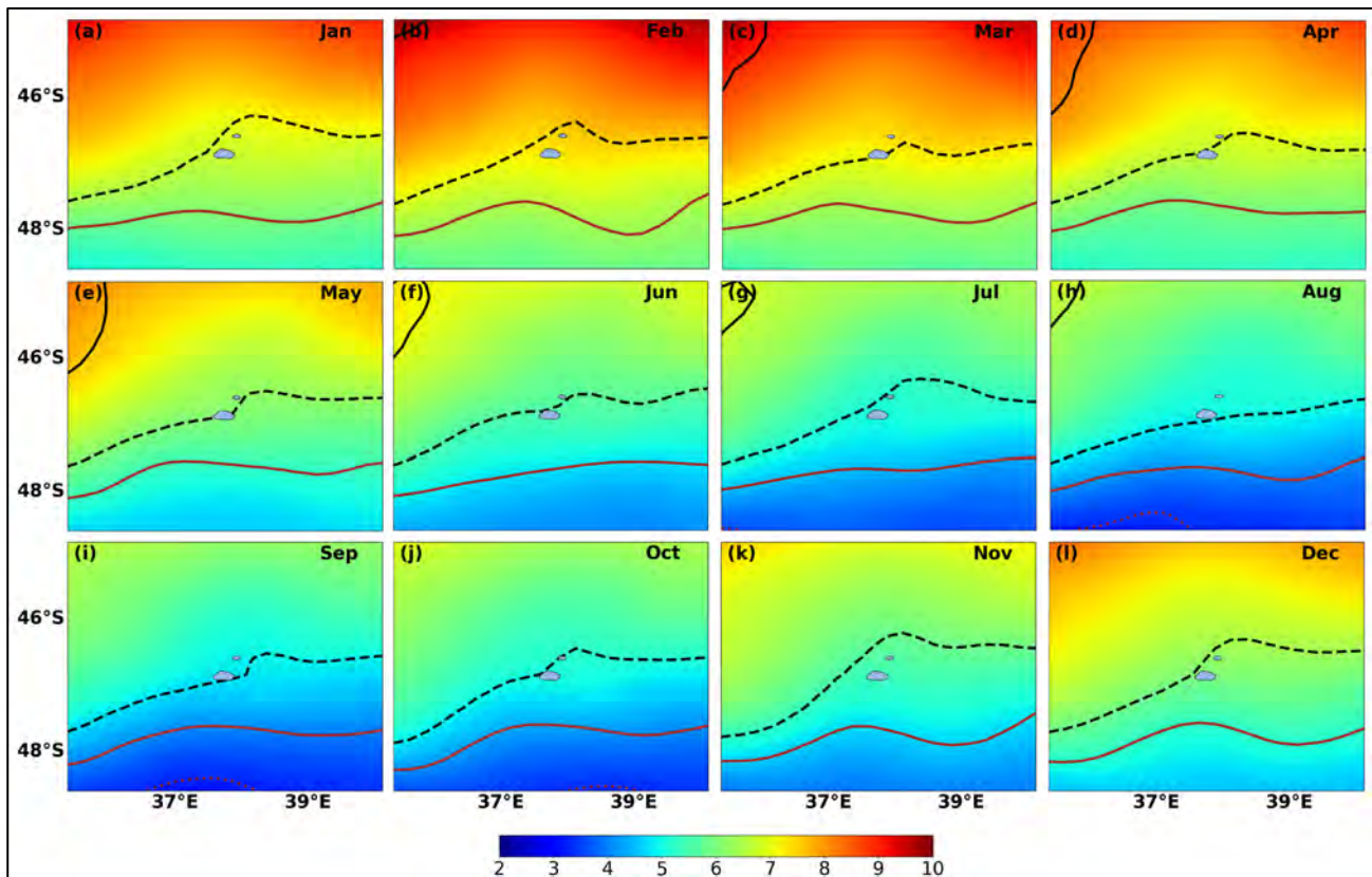
Figure 2: Monthly climatology of sea surface temperature ( ^{\circ}\text{C} ) around the PEIs. The solid/dashed black lines show the positions of middle/southern branches of the sub-Antarctic Front (M-SAF/S-SAF), and the solid/dotted brown lines indicate the northern/middle branches of the Antarctic Polar Front (N-APF/M-APF)
