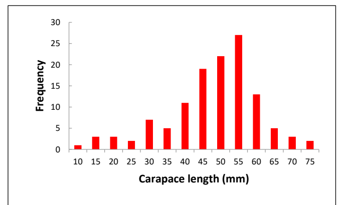
Figure 3: Frequency of carapace lengths in different size classes of West Coast rock lobster found in pellets regurgitated by bank cormorants in South Africa, 1975–2002
