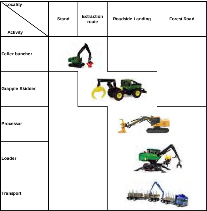
Figure 5-8: Multi-Stem Harvesting System
