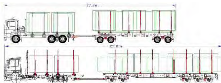
Figure 2-7: Baseline (top) and Performance-Based Standards (below)
