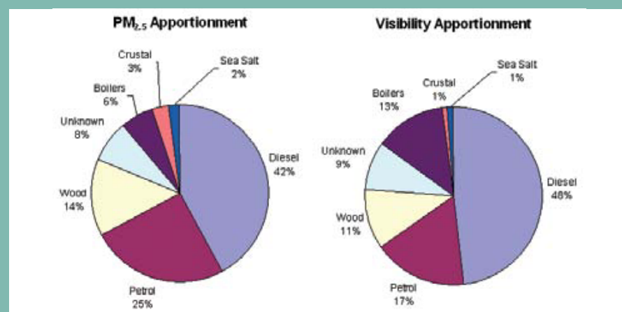
Figure 9.1: To gather information about the quality required for satisfactory modelling, data for six brown haze episodes were used in the Chemical Mass Balance Model to determine the contribution of various sources to Cape Town's brown haze. This figure shows PM_{2.5} apportionments (left) and the contribution of each source to impairment of visibility (right) (Wicking-Baird et al. , 1997).
