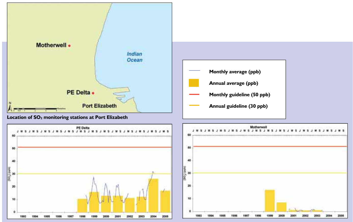
Figure 4.2.3.2: Long-term trends in SO 2 levels at Port Elizabeth
