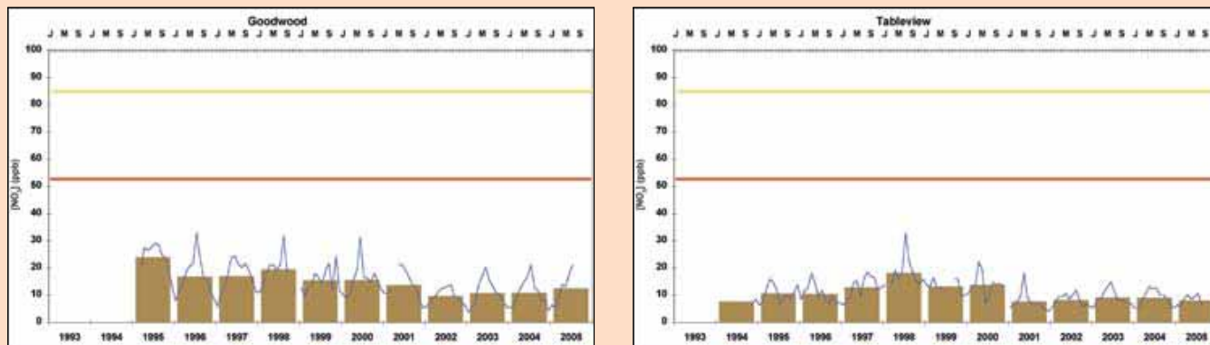
Figure 4.2.2.1: Long-term \text{NO}_2 trends at Cape Town
