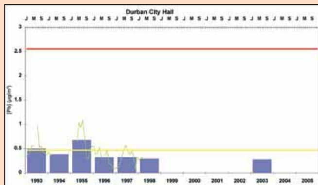
Figure 4.2.4.3: Trends in Pb levels in KwaZulu-Natal
