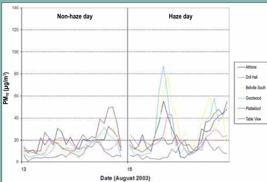
Figure 9.2: Comparison of ground-based PM 10 measurements between a non-haze day (13 August 2003) (left) and a haze day (15 August 2003) (right). The data are represented on a time series starting at midnight
