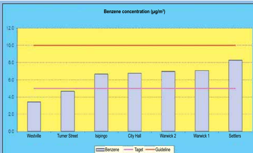
Figure 7.4: Benzene concentrations in Durban, 2004 Source: eThekweni Annual Report, 2004
