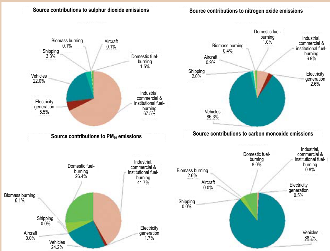
Figure 4.9: Contributions of different emission sources affecting Cape Town
