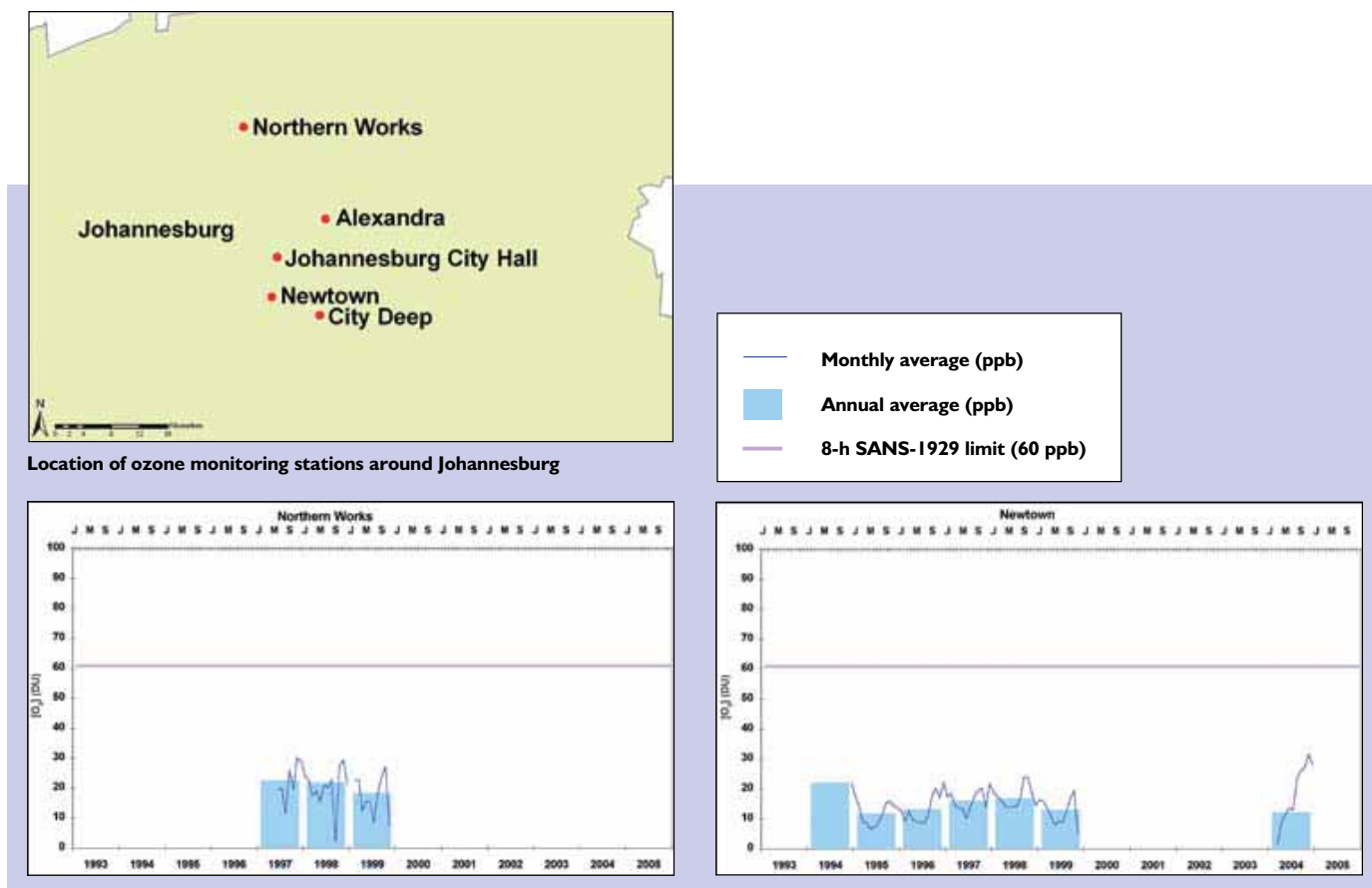
Figure 4.2.1.3: Long-term trend of ozone levels around Johannesburg
