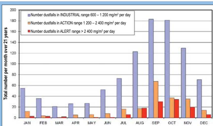
Figure 7.12: Number of dustfall measurements recorded on the Central Witwatersrand during the period 1985–2005 that are in 'industrial', 'action' and 'alert' ranges
