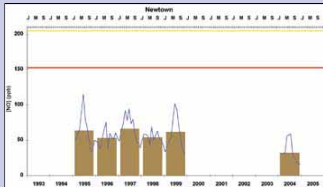
Figure 4.2.2.4: Long-term trends in NO concentration levels in Gauteng and Mpumalanga
