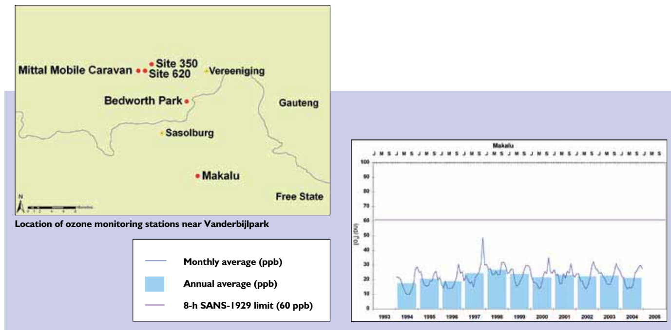
Figure 4.2.1.5: Long-term trend of ozone levels near Vanderbijlpark
