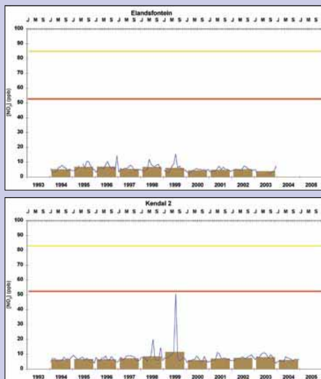
Figure 4.2.2.2: Long-term trend in \text{NO}_2 levels in Gauteng and Mpumalanga
