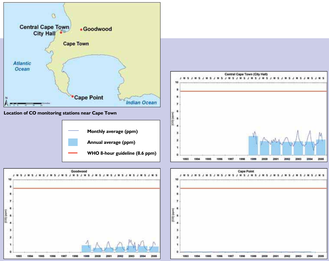
Figure 4.2.5.1: Trends in CO levels near Cape Town
