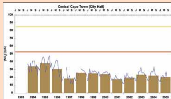
Figure 4.2.2.1: Long-term \text{NO}_2 trends at Cape Town
