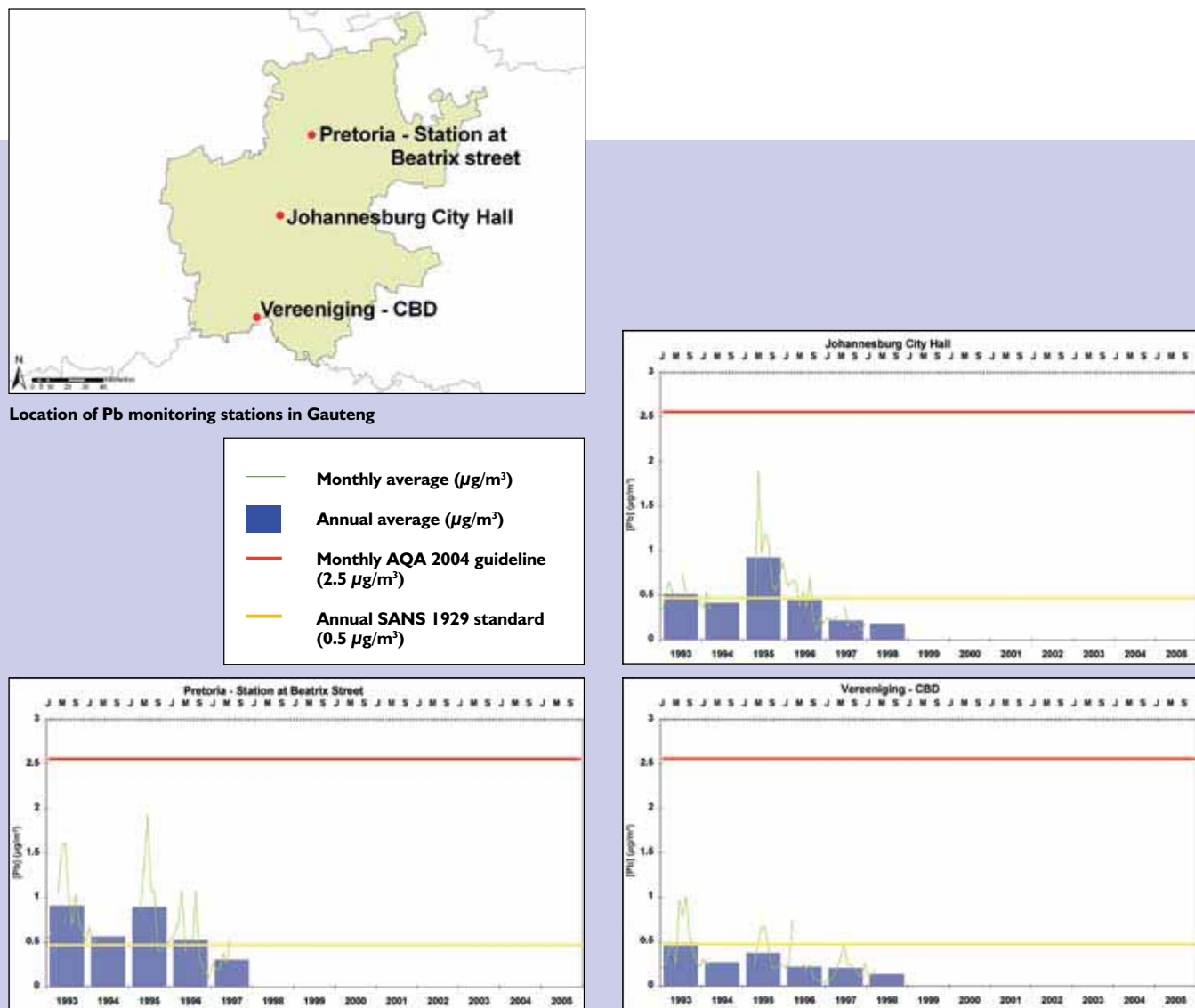
Figure 4.2.4.2: Trends in lead levels in Gauteng
