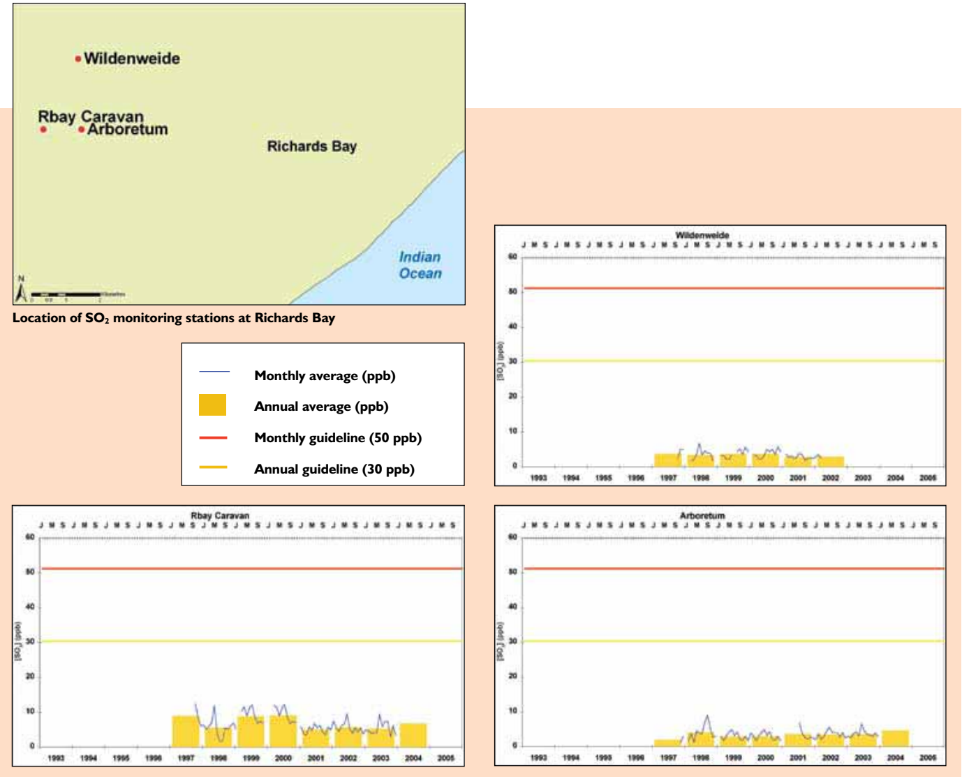
Figure 4.2.3.5: Long-term SO 2 levels at Richards Bay
