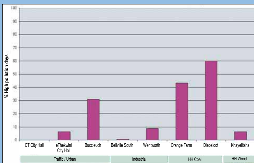
Figure 7.3: Frequency of occurrence of high pollution days due to fine inhalable particulate concentrations of \text{PM}_{10} at selected sites, 2004
