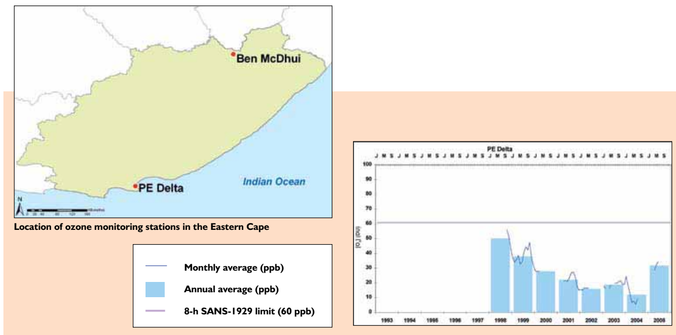
Figure 4.2.1.2: Long-term trend of ozone levels in the Eastern Cape
