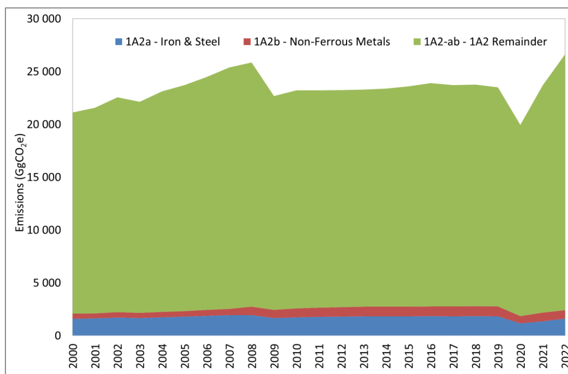
Figure 3.11: 1A2 Disaggregated emissions 2000 - 2022
