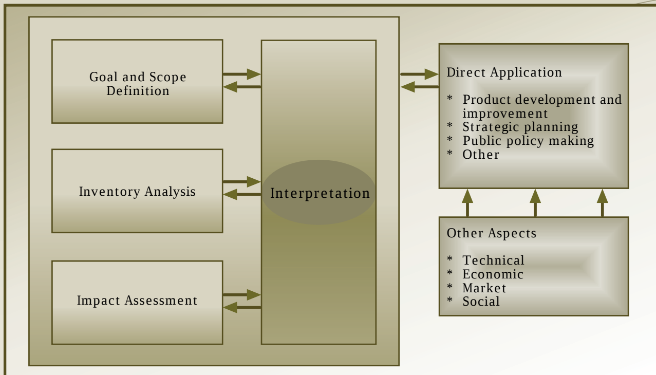
Figure 2: Illustration of Life Cycle Assessment Procedure
