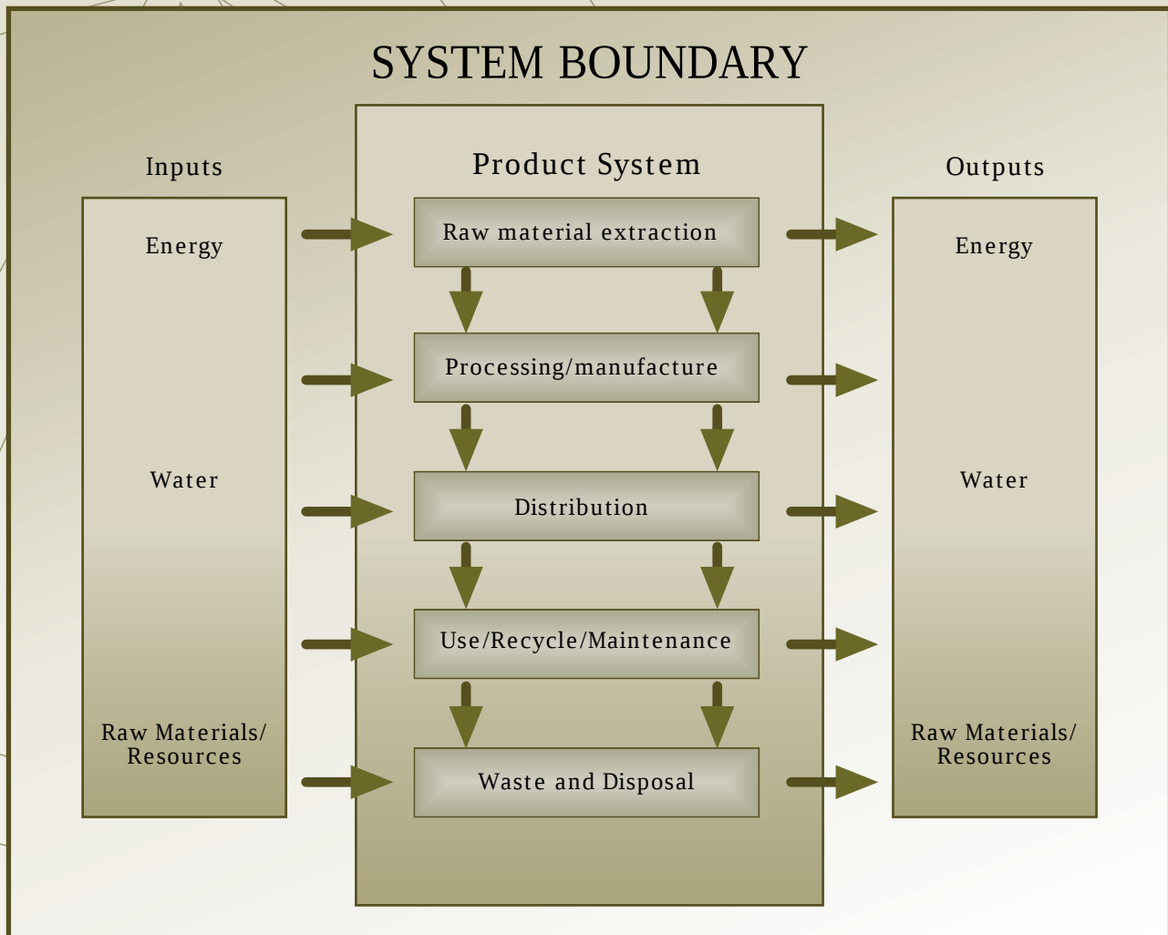
Figure 1: Life Cycle Assessment framework based on the ISO 14040 model
