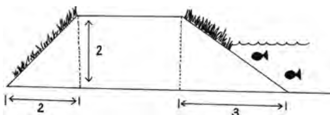
Suggested ratios of pond walls.
