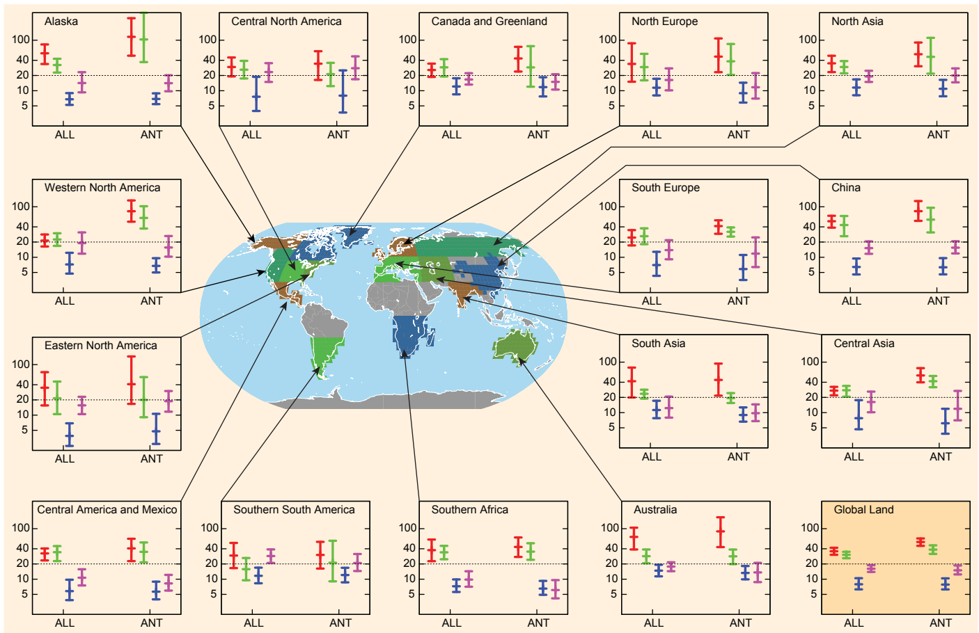
Figure 3-2 | Estimated return periods (years) and their 5 and 95% uncertainty limits for 1960s 20-year return values of annual extreme daily temperatures in the 1990s climate (see text for more details). ANT refers to model simulated responses with only anthropogenic forcing and ALL is both natural and anthropogenic forcing. Error bars are for annual minimum daily minimum temperature (red: T Nn ), annual minimum daily maximum temperature (green: T Xn ), annual maximum daily minimum temperature (blue: T Nx ), and annual maximum daily maximum temperature (pink: T Xx ), respectively. Grey areas have insufficient data. Source: Zwiers et al., (2011).
