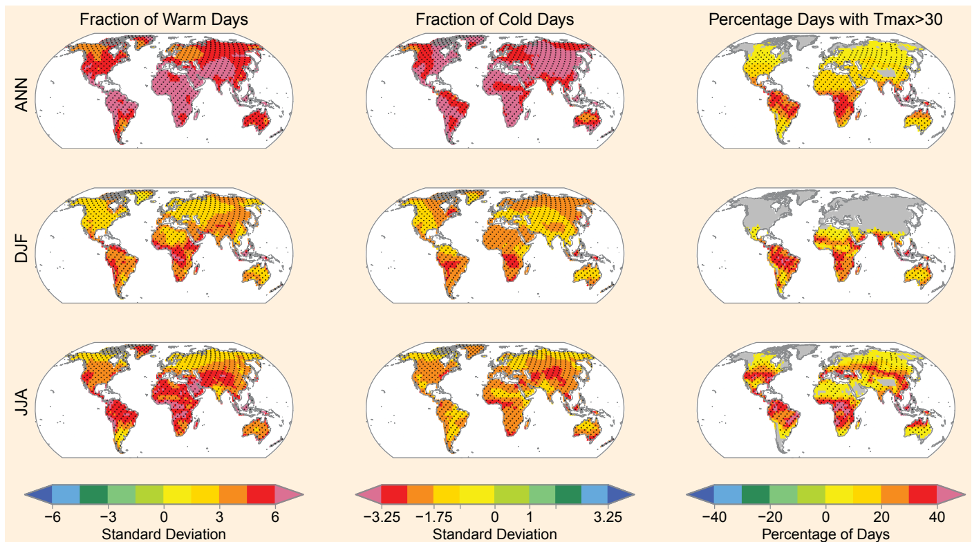
Figure 3-3 | Projected annual and seasonal changes in three indices for daily Tmax for 2081-2100 with respect to 1980-1999, based on 14 GCMs contributing to the CMIP3. Left column: fraction of warm days (days in which Tmax exceeds the 90th percentile of that day of the year, calculated from the 1961-1990 reference period); middle column: fraction of cold days (days in which Tmax is lower than the 10th percentile of that day of the year, calculated from the 1961-1990 reference period); right column: percentage of days with Tmax > 30°C. The changes are computed for the annual time scale (top row) and two seasons (December-January-February, DJF, middle row, and June-July-August, JJA, bottom row) as the fractions/percentages in the 2081-2100 period (based on simulations for emission scenario SRES A2) minus the fractions/percentages of the 1980-1999 period (from corresponding simulations for the 20th century). Warm day and cold day changes are expressed in units of standard deviations, derived from detrended per year annual or seasonal estimates, respectively, from the three 20-year periods 1980-1999, 2046-2065, and 2081-2100 pooled together. Tmax > 30°C changes are given directly as differences in percentage points. Color shading is only applied for areas where at least 66% (i.e., 10 out of 14) of the GCMs agree on the sign of the change; stippling is applied for regions where at least 90% (i.e., 13 out of 14) of the GCMs agree on the sign of the change. Adapted from Orłowsky and Seneviratne (2011); updating Tebaldi et al. (2006) for additional number of indices and CMIP3 models, and including seasonal time frames. For more details, see Appendix 3.A.
