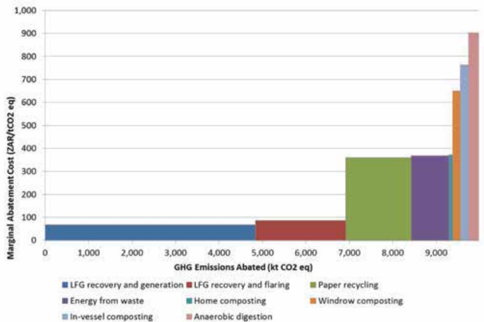
Figure 51: Marginal abatement cost curve for the waste sector in 2020
