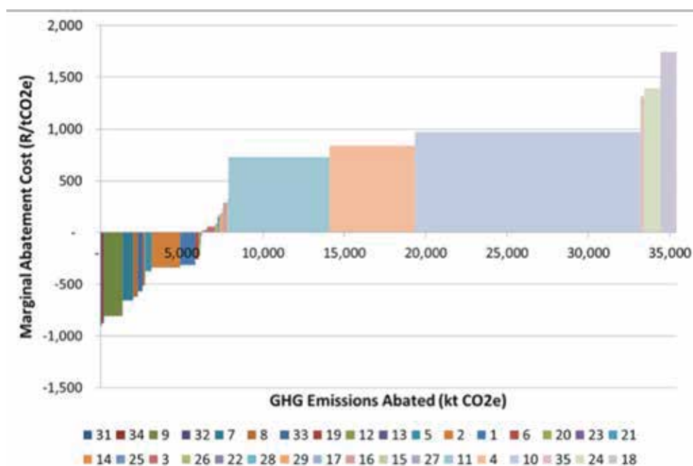
Figure 18: Marginal abatement cost curve for the non-power sector in 2030
