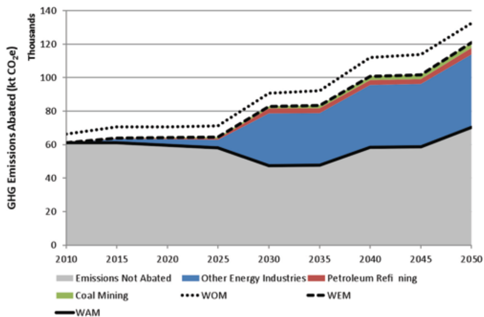
Figure 21: WAM scenario for the non-power sector, showing a breakdown between subsectors. Emissions from the power sector have been reallocated to end users and electricity related emissions savings have been adjusted accordingly. Reference case WOM and WEM emission projections are also shown.
