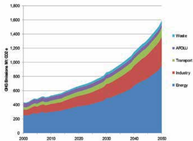
Figure 7: National GHG emissions under the reference case WEM projection, showing a breakdown per sector (2000–2050)
