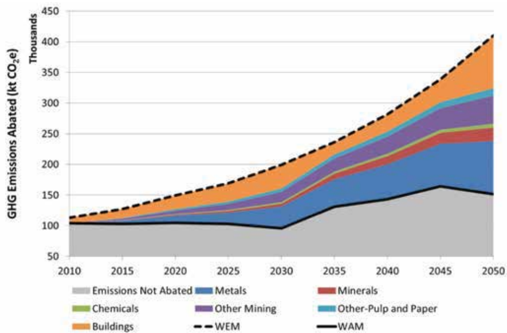
Figure 40: WAM scenario for the industry sector, showing a breakdown per sector. Emissions from the power sector have been reallocated to end-use sectors and electricity-related emissions savings have been adjusted accordingly. The reference case WEM emission projection is also shown
