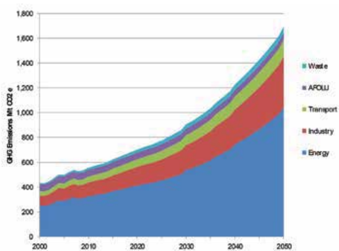
Figure 5: National GHG emissions under the reference case WOM projection, showing a breakdown per sector (2000–2050)
