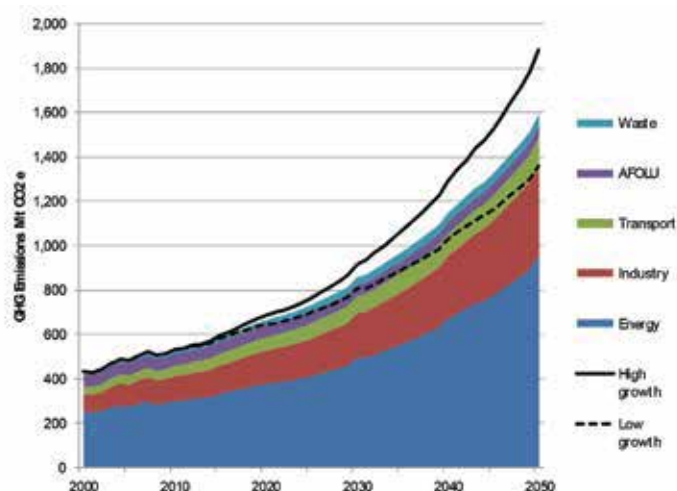
Figure 9: National GHG emissions under the reference case WEM projection, showing high and low growth compared to medium growth (2000–2050)
