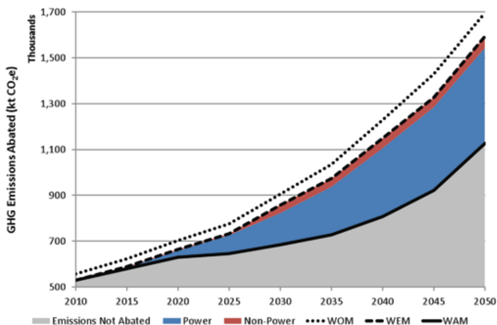
Figure 20: WAM scenario for the energy sector, showing a breakdown between the power and non-power sectors. Emissions from the power sector have been reallocated to end users and electricity related emissions savings have been adjusted accordingly. Reference case WOM and WEM emission projections are also shown.
