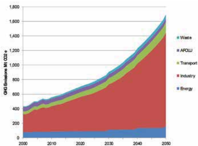
Figure 6: National GHG emissions under the reference case WOM projection, showing a breakdown per sector (2000–2050), with electricity emissions allocated to end use sectors
