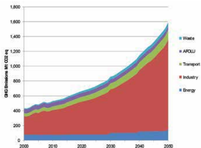
Figure 8: National GHG emissions under the reference case WEM projection, showing a breakdown per sector (2000–2050), with electricity emissions allocated to end use sectors
